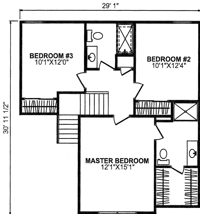
SECOND FLOORPLAN
