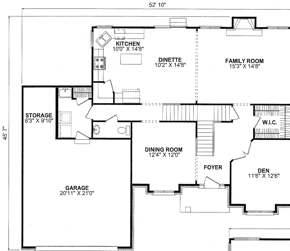
FIRST FLOORPLAN
