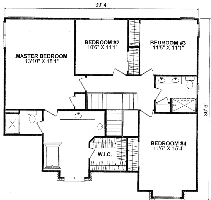
SECOND FLOORPLAN
