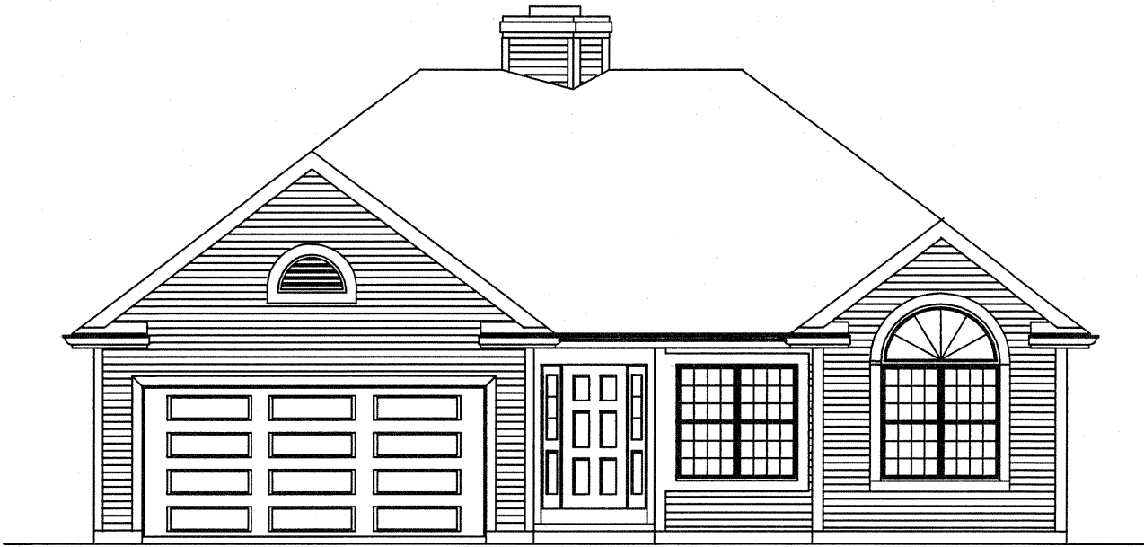
STANDARD FRONT ELEVATION
