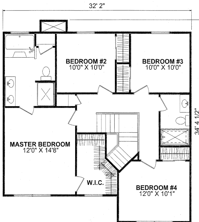
SECOND FLOORPLAN
