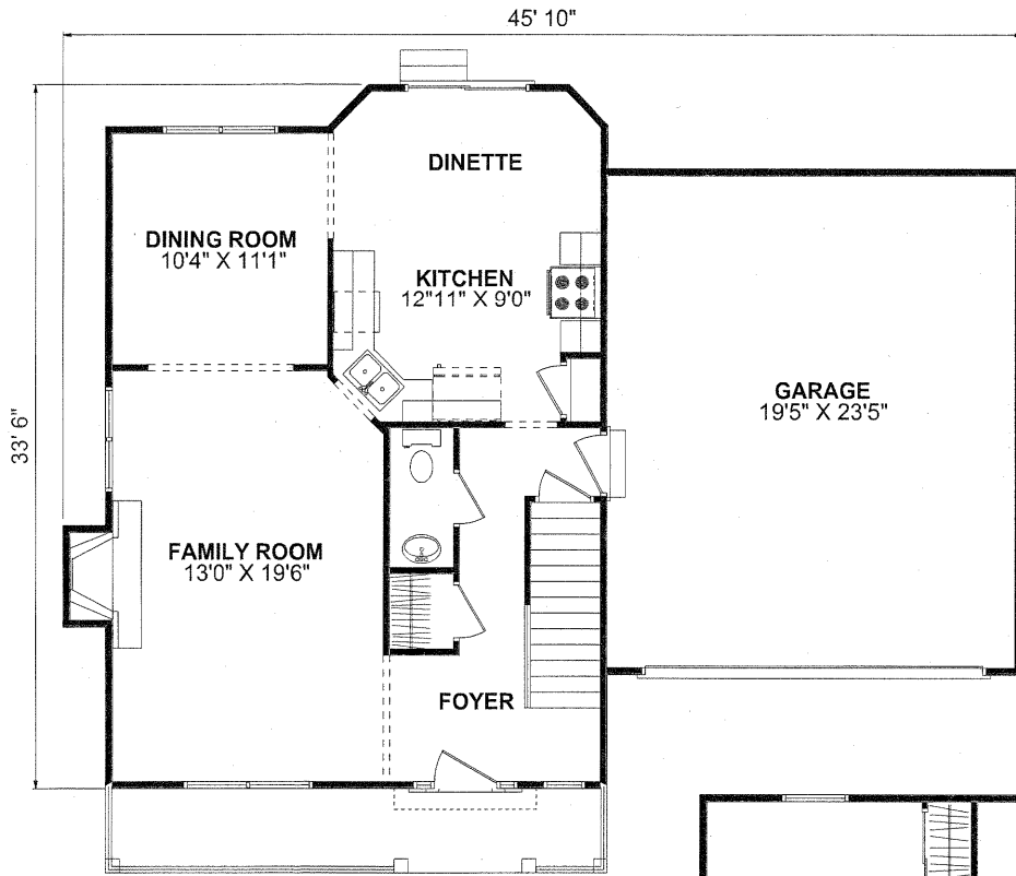
FIRST FLOORPLAN
