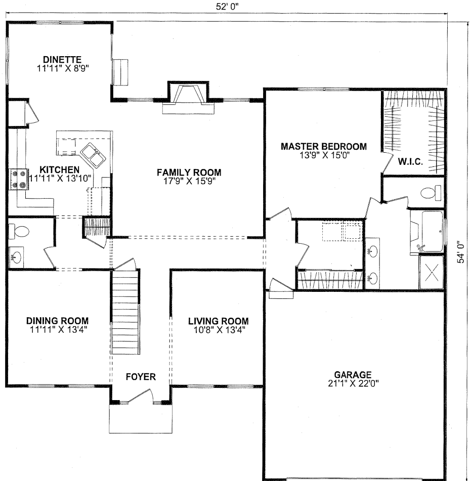
FIRST FLOORPLAN
