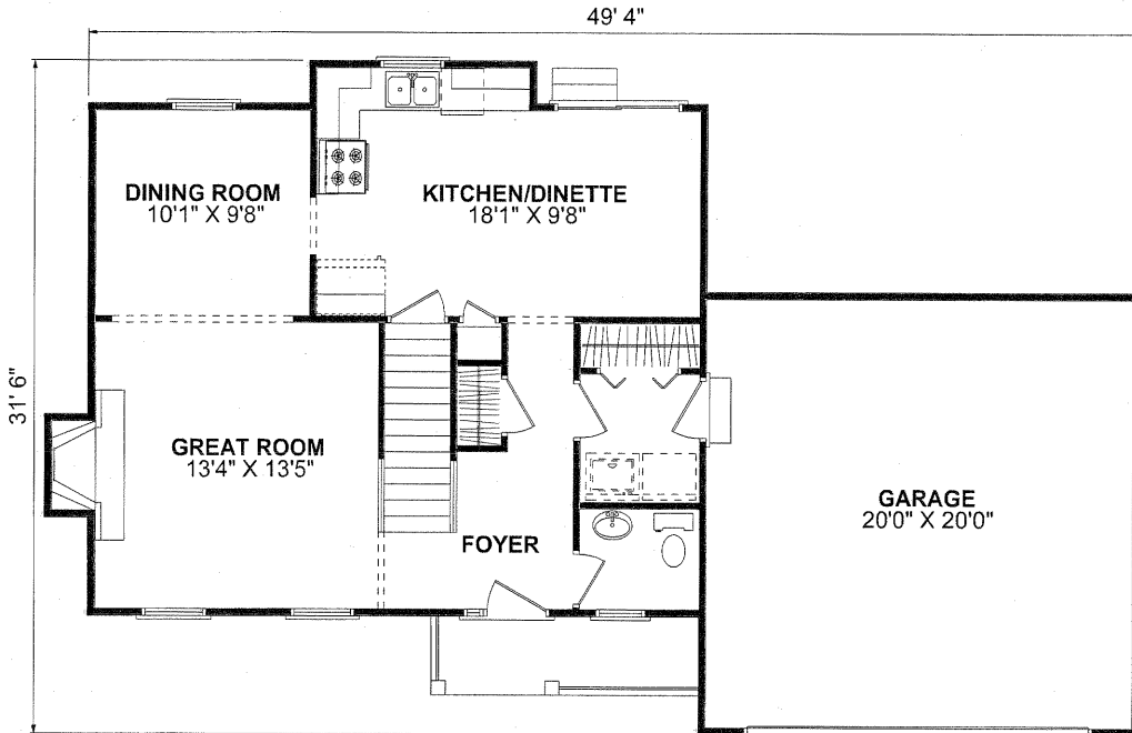
FIRST FLOORPLAN
