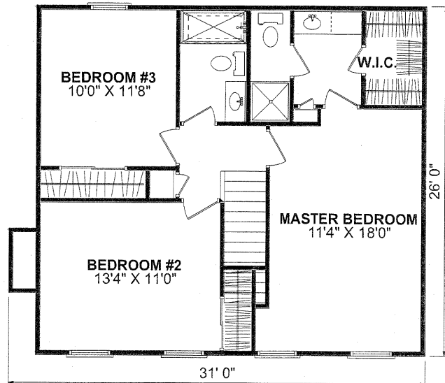
SECOND FLOORPLAN
