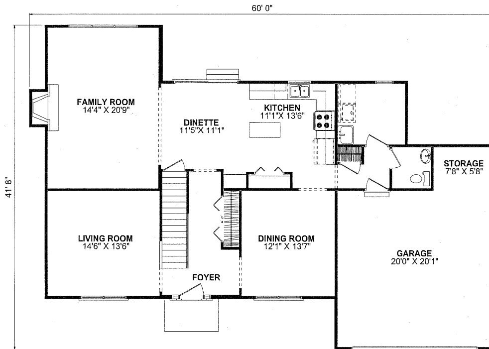
FIRST FLOORPLAN
