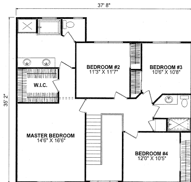
SECOND FLOORPLAN
