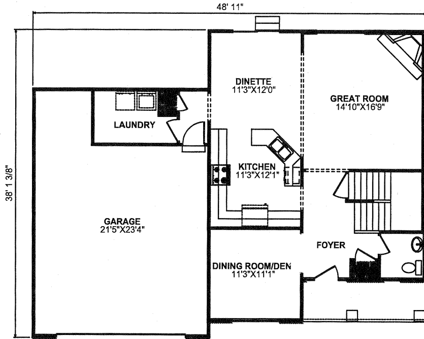
FIRST FLOORPLAN
