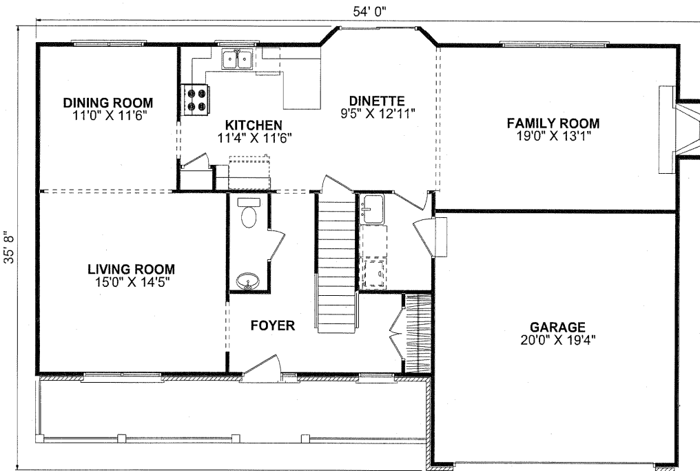
FIRST FLOORPLAN
