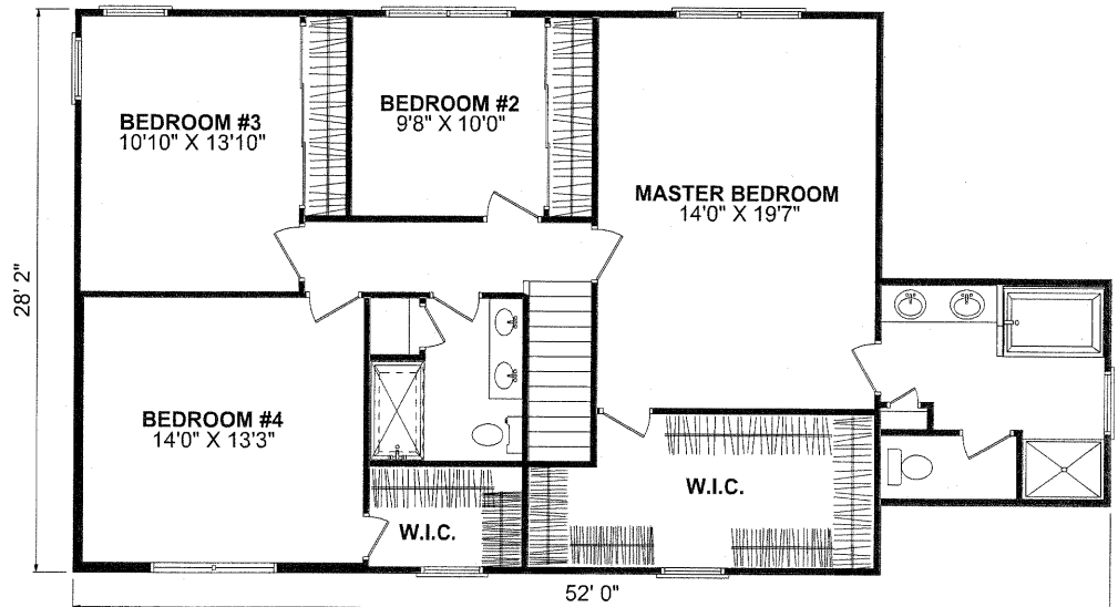
SECOND FLOORPLAN
