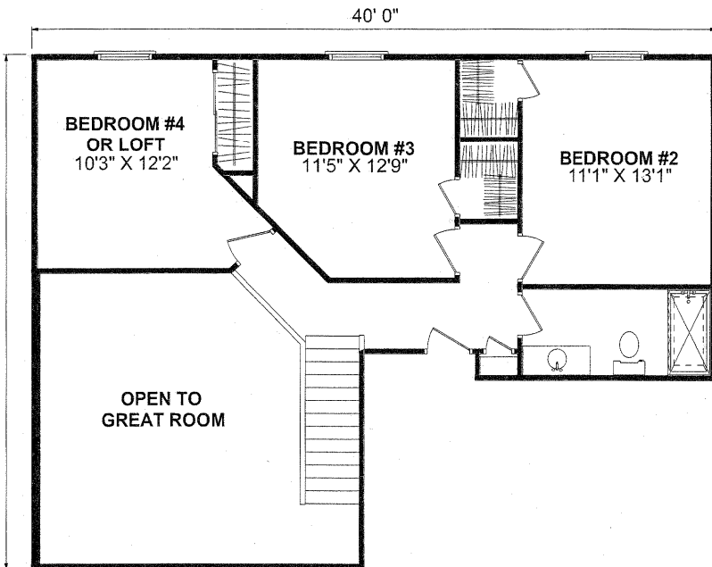
SECOND FLOORPLAN
