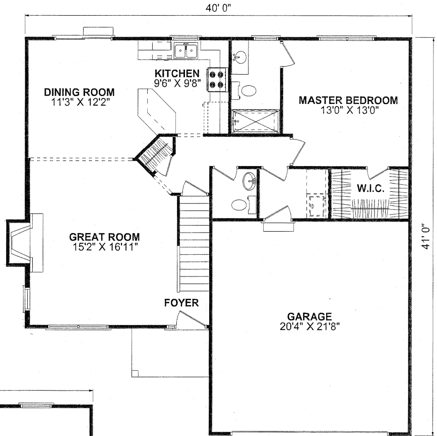
FIRST FLOORPLAN
