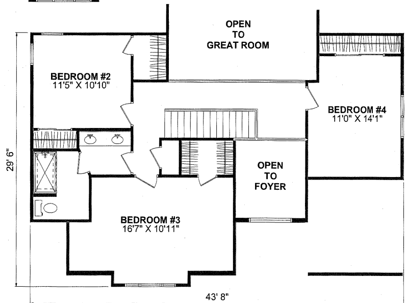
SECOND FLOORPLAN
