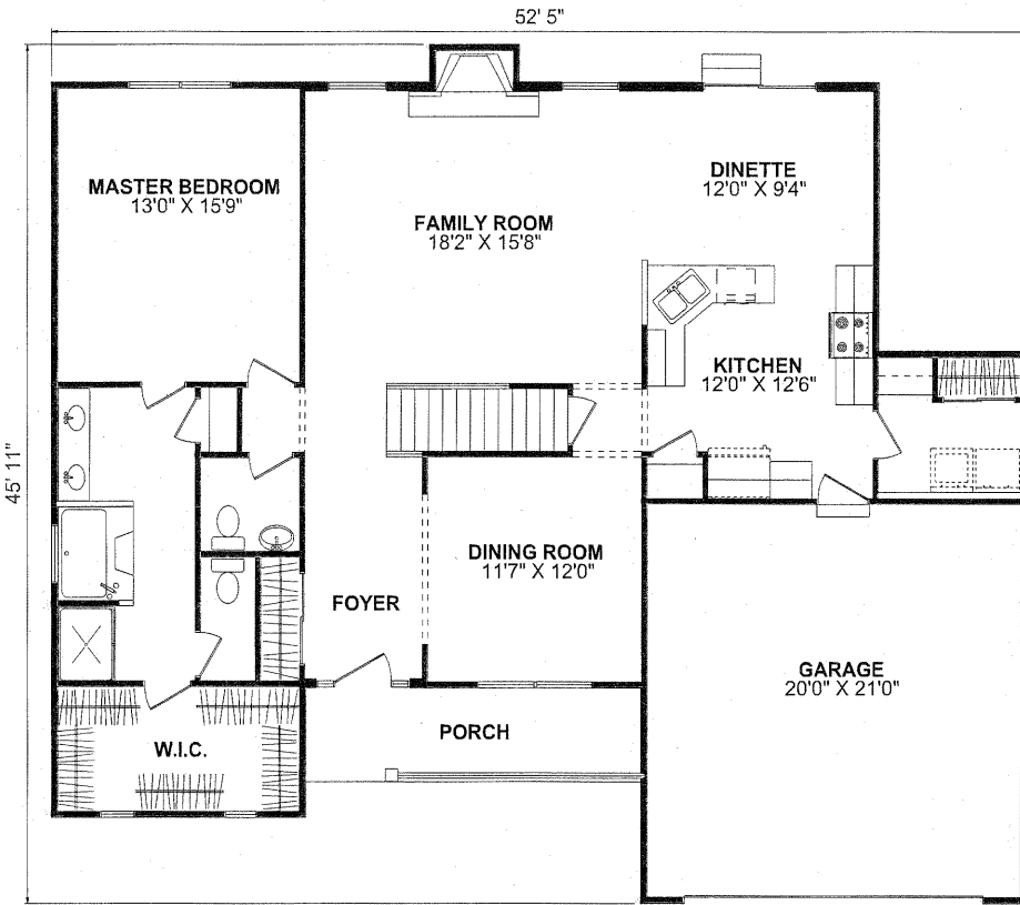
FIRST FLOORPLAN
