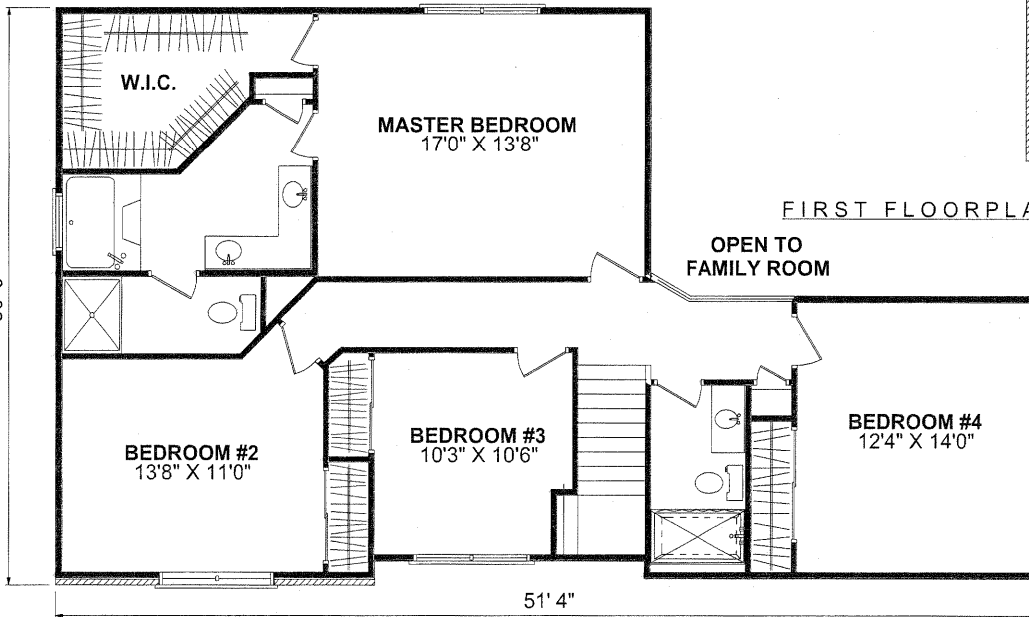
SECOND FLOORPLAN
