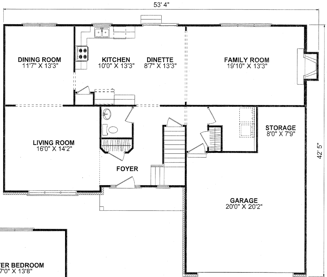
FIRST FLOORPLAN
