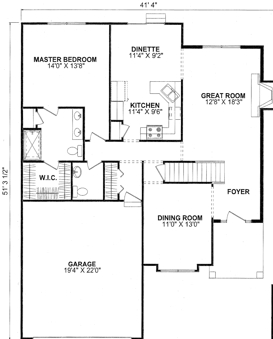
FIRST FLOORPLAN
